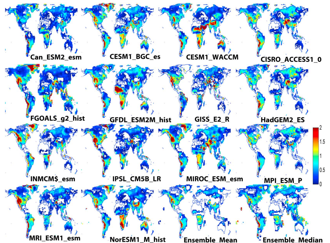
Figure 2. Quantile bias ( t = 75 percentile, QB_{75} with optimal value = 1) maps for selected CMIP5 precipitation simulations, and for their ensemble mean and median, all with respect to GPCP observations.
